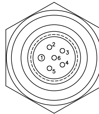
SOLDER CUP VIEW
