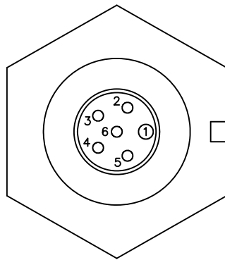
PIN VIEW
